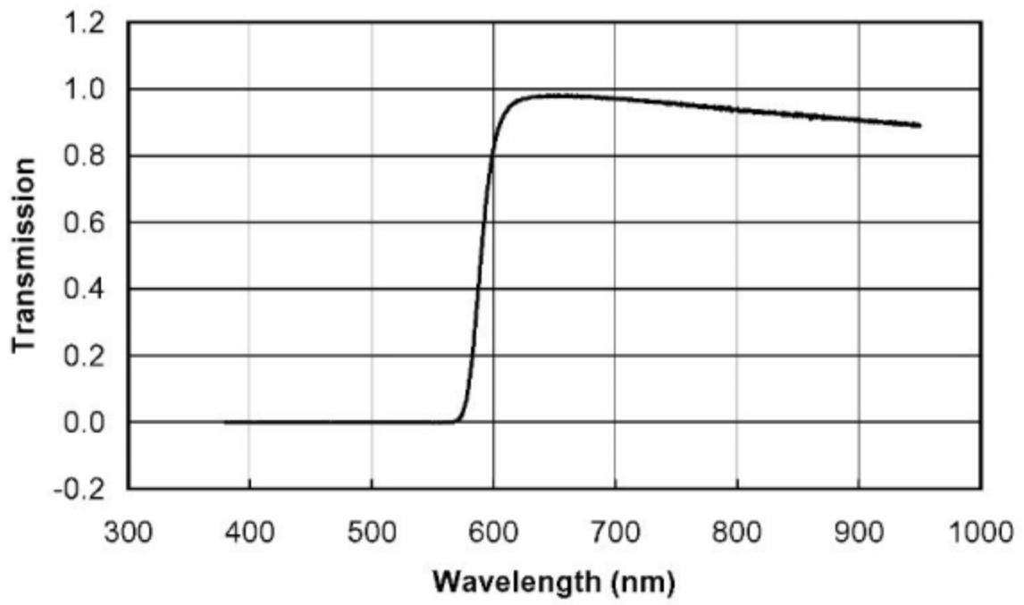
LDSS OG590 Filter Throughput
